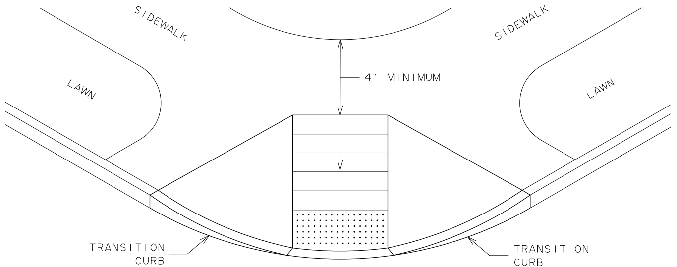
ACCESS RAMP TYPE A
