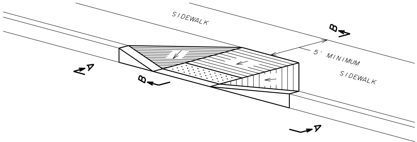
ACCESS RAMP TYPE B ISOMETRIC
