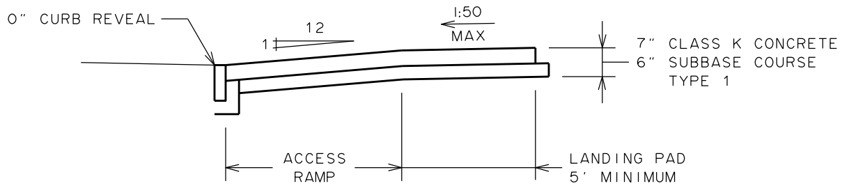
SECTION B-B
