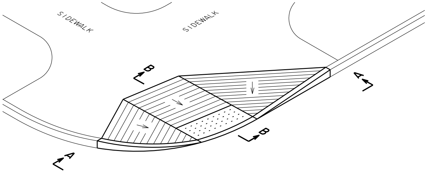
ACCESS RAMP TYPE D ISOMETRIC
