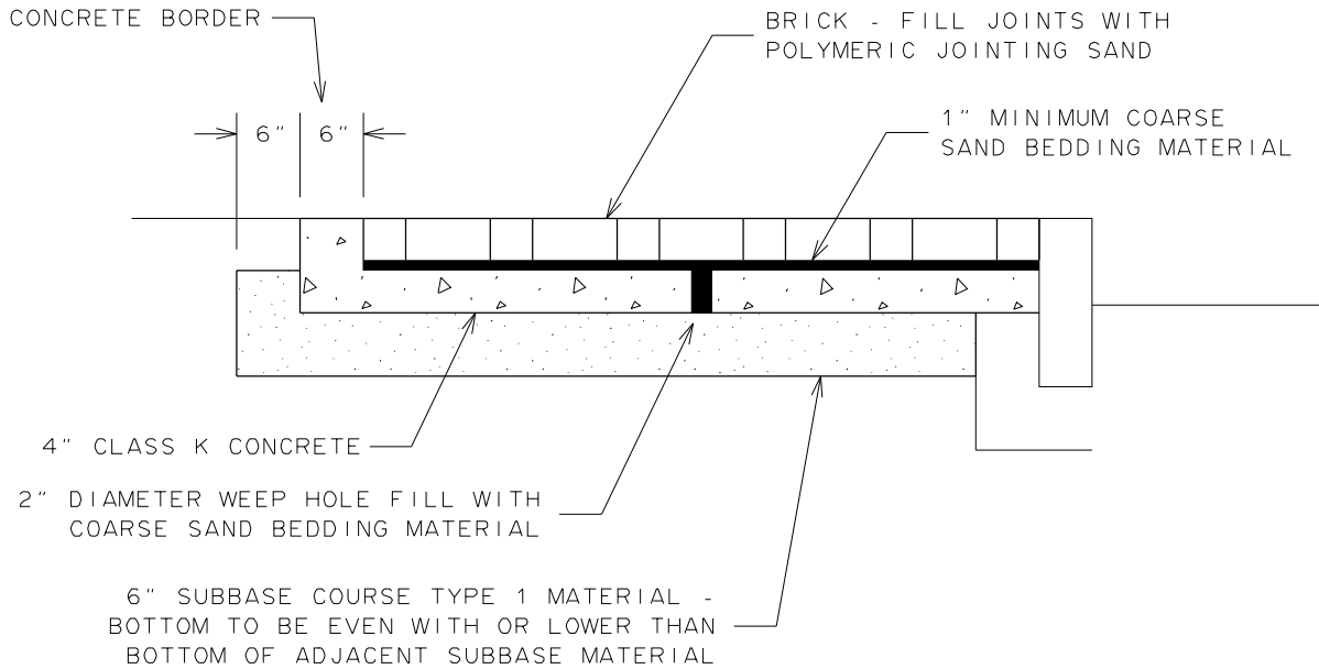
OPTIONAL CONCRETE FOUNDATION
