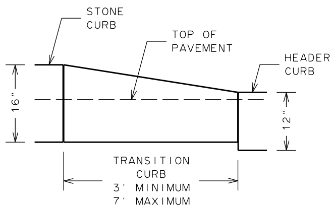
TRANSITION CURB
