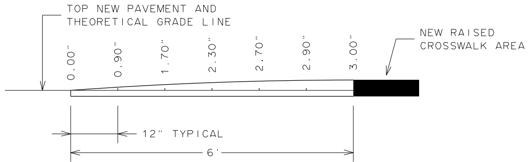
CROSS-SECTION APPROACH RAMP
