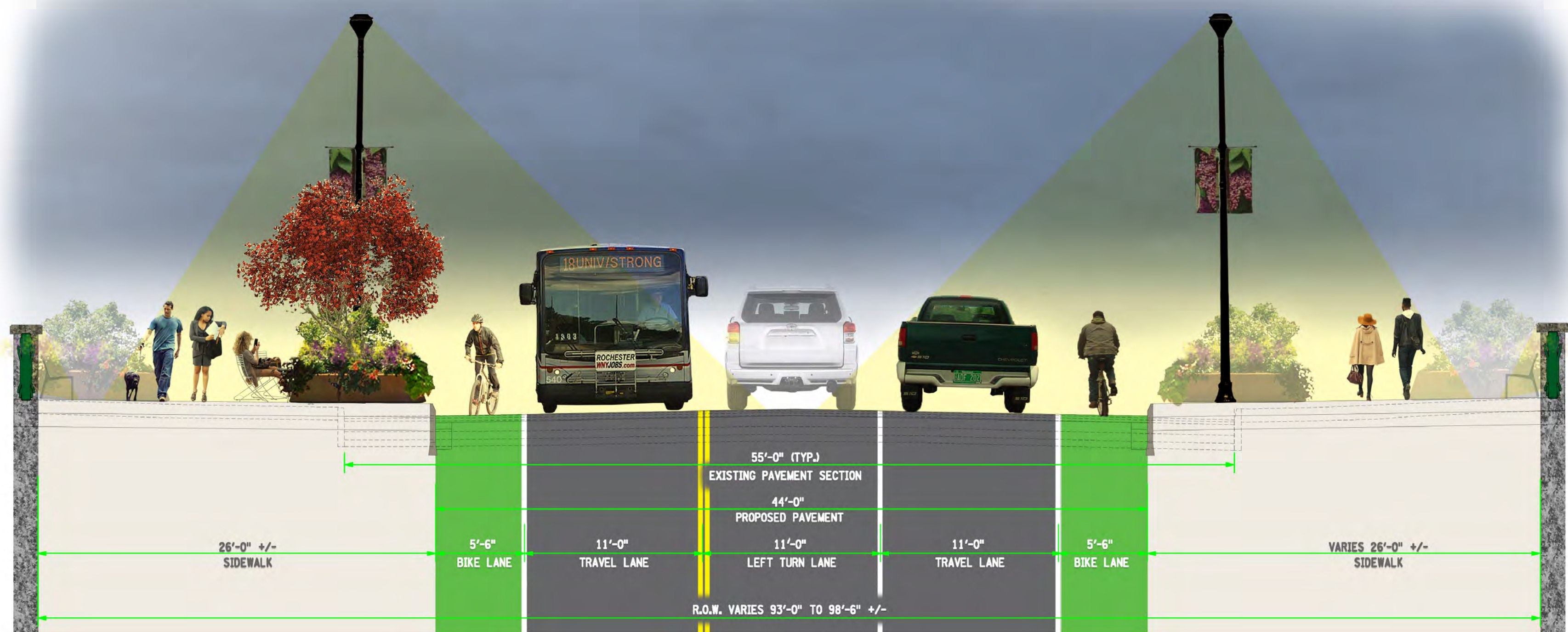
SECTION B-B BRIDGE - LOOKING EAST
