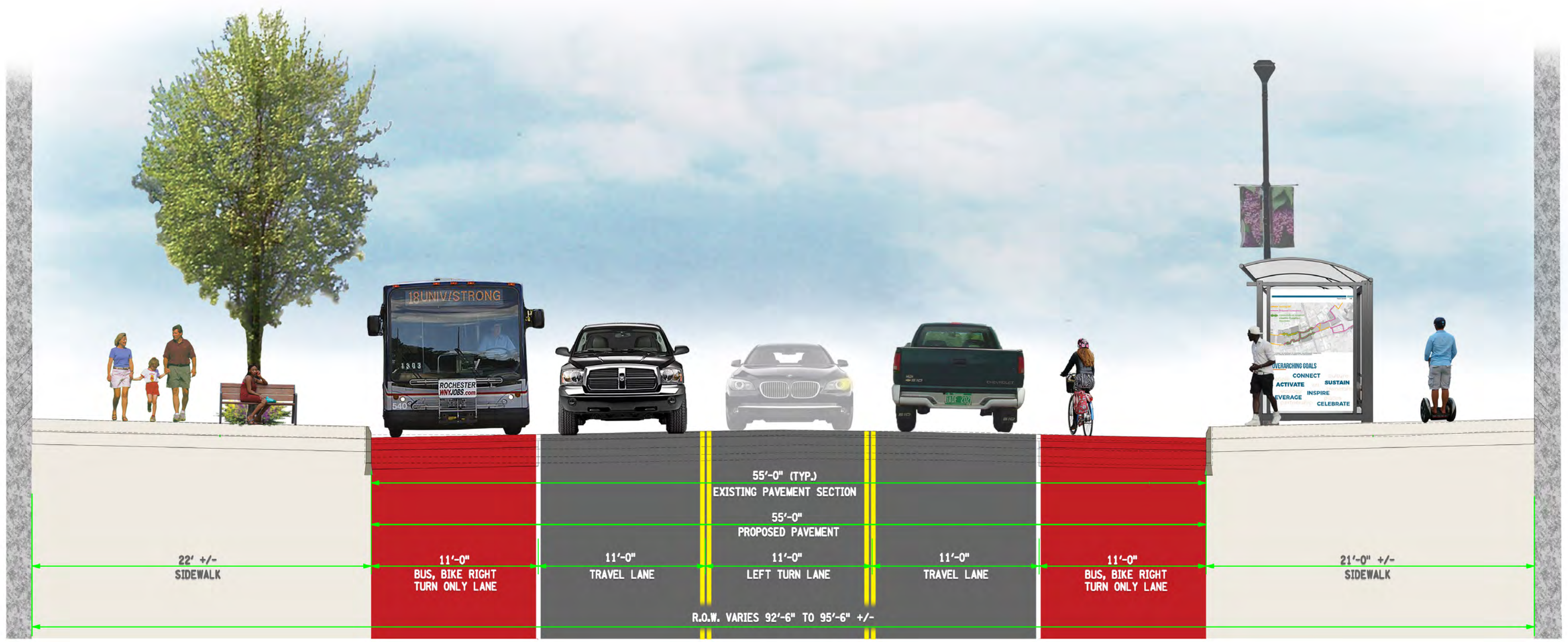
SECTION A-A WEST SIDE - LOOKING EAST
