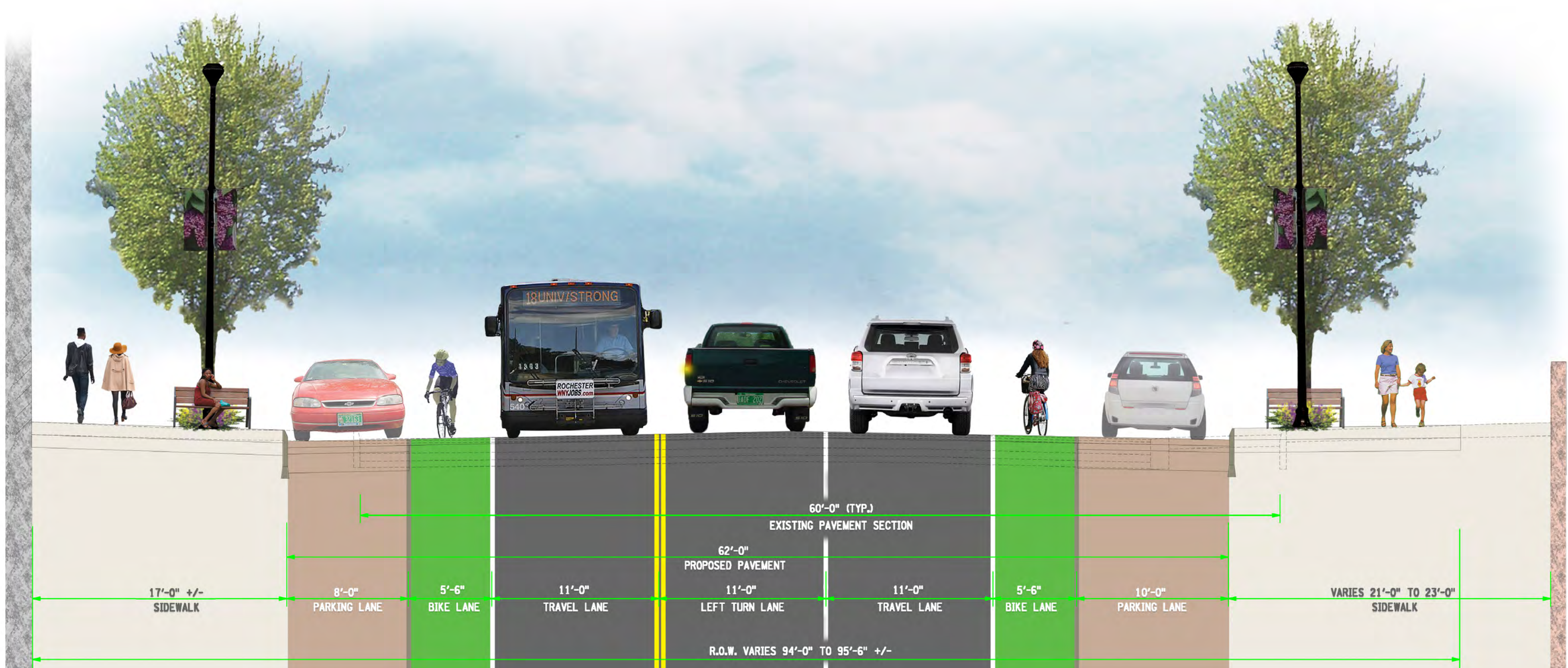
SECTION C-C EAST SIDE - LOOKING EAST
