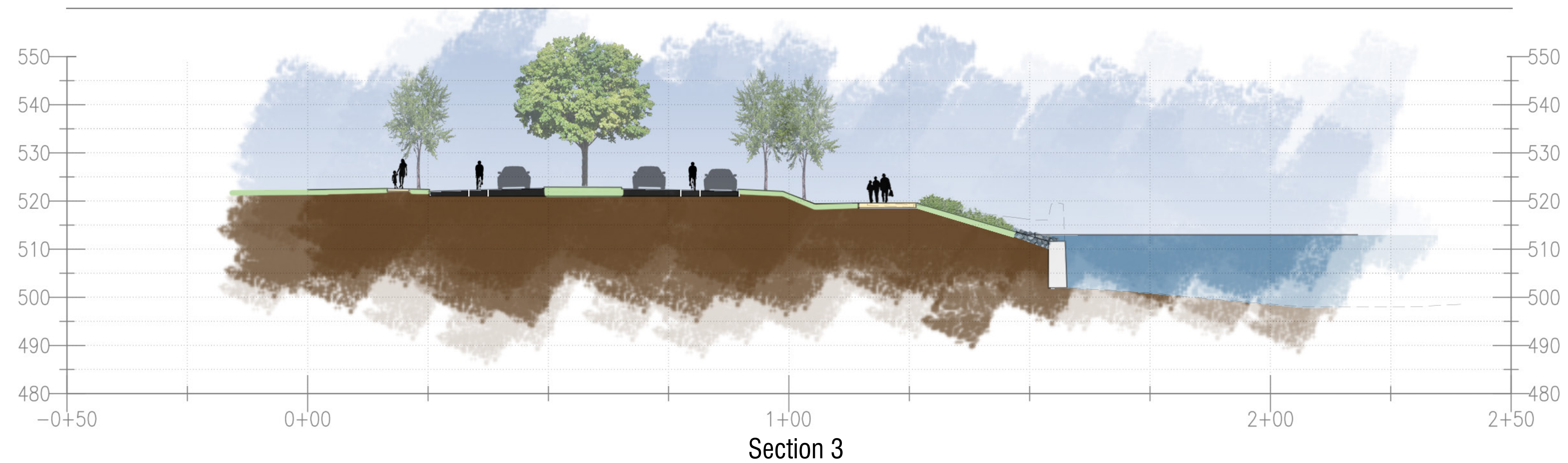
West River Wall - Concept Sections
