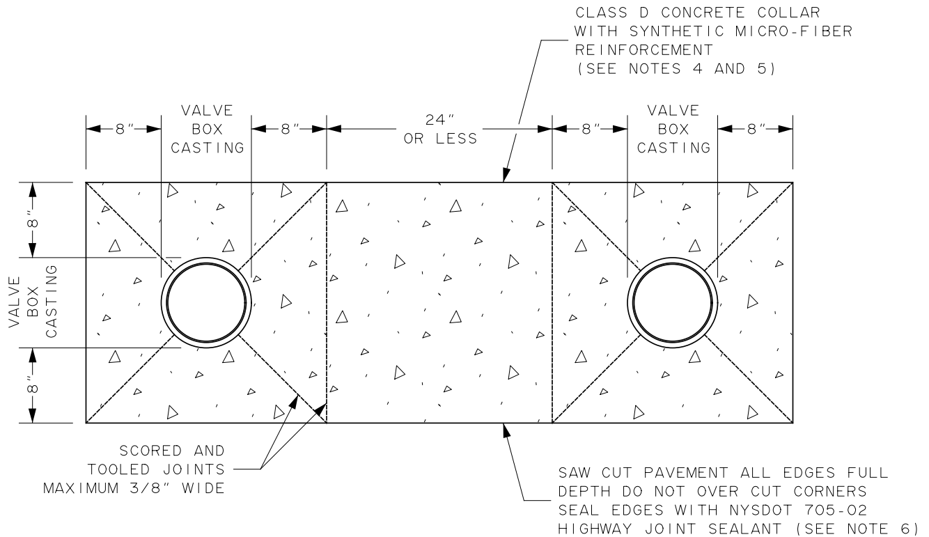
PLAN (FOR SECTION VIEW SEE DETAIL S909-3)
