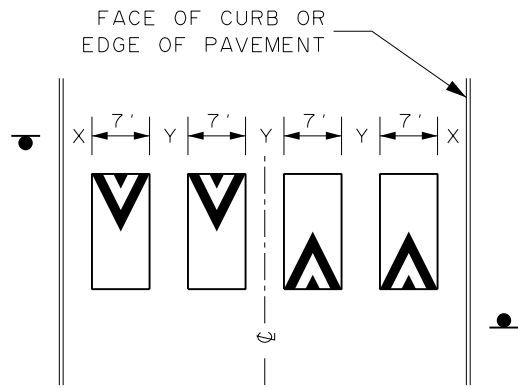
4 SPEED CUSHION LAYOUT
