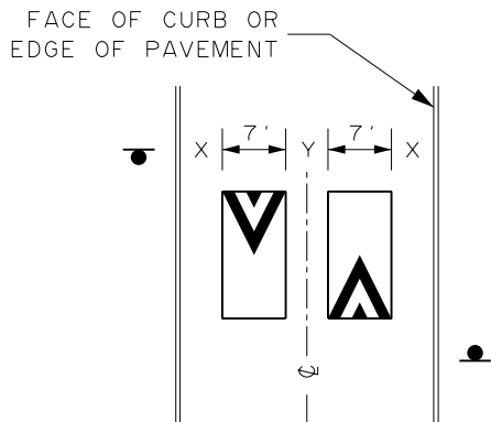
2 SPEED CUSHION LAYOUT
