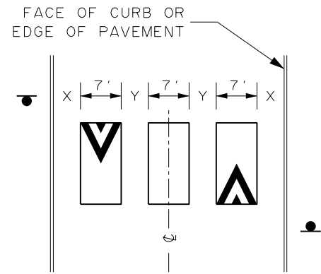
3 SPEED CUSHION LAYOUT
