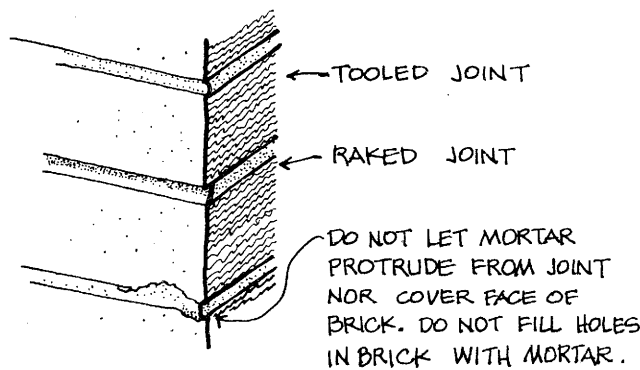
MASONRY
