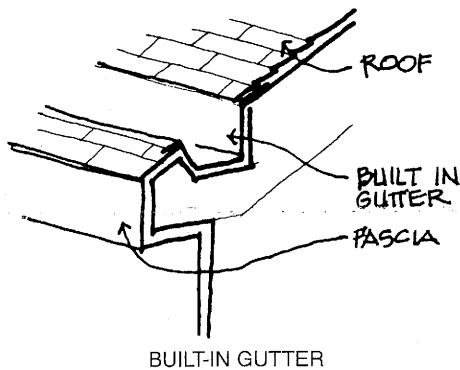
BUILT-IN GUTTER
