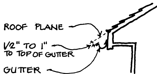
GUTTER LOCATION
