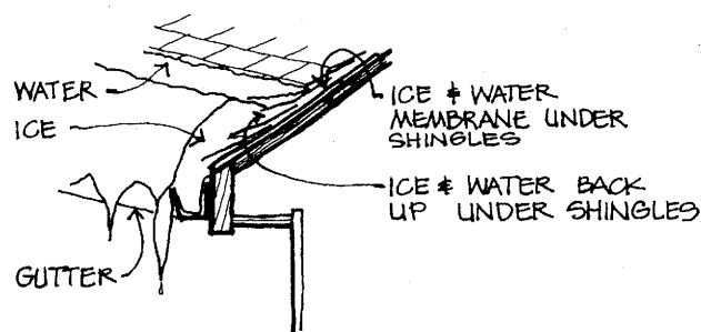
ICE DAM
