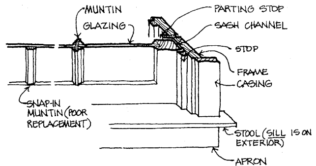
WINDOW ELEMENTS
