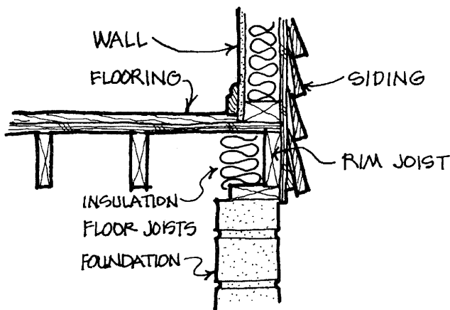
INSULATING THE RIM JOIST
