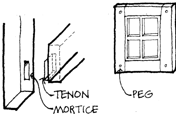
MORTICE & TENON
