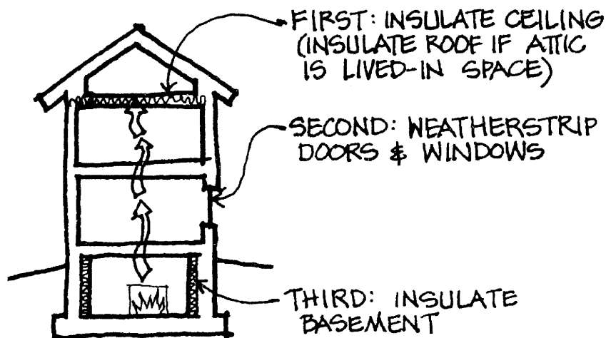
INSULATION PRIORITIES
