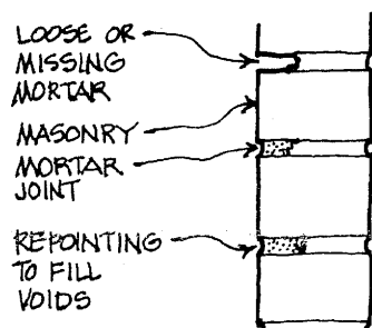
REPOINTING
