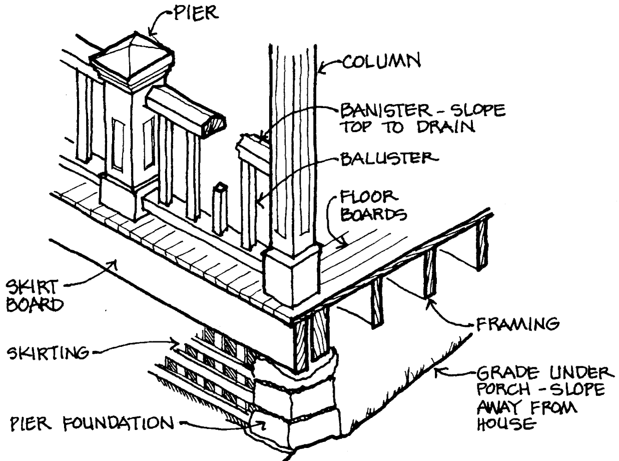
PORCH ELEMENTS
