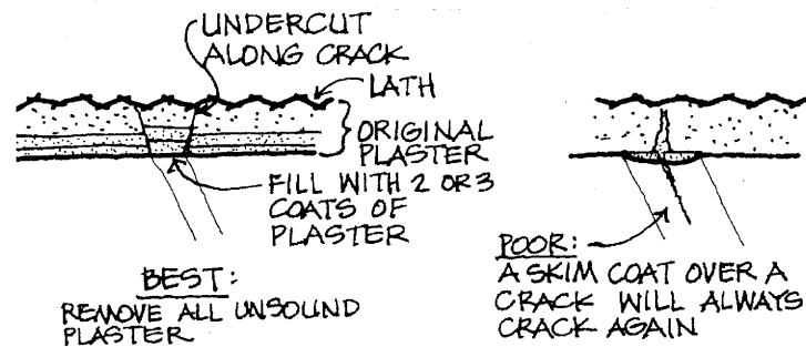
PLASTER REPAIR
