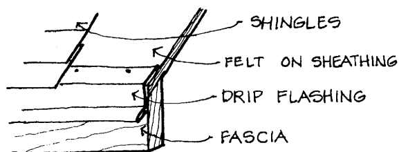
DRIP FLASHING
