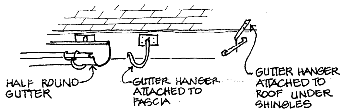
HALF-ROUND GUTTER
