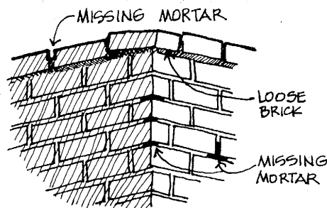
CHIMNEY MASONRY
