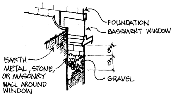
WINDOW WELL
