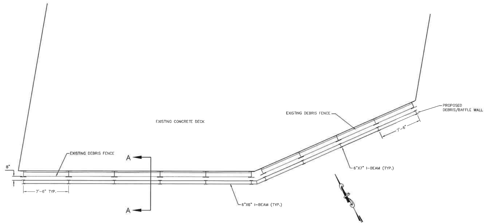
PLAN VIEW SOUTH SIDE RECONSTRUCTED DEBRIS/BAFFLE WALL SCALE: 1/4" = 1'-0"
