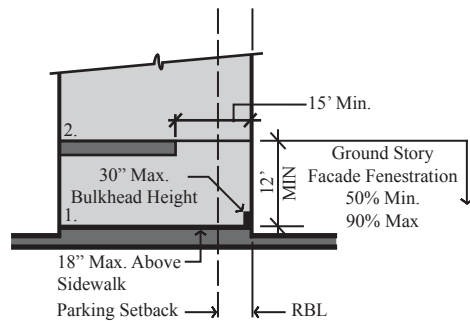
COMMERCIAL FRONTAGE
