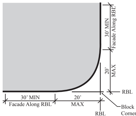
ROUNDED CORNER
