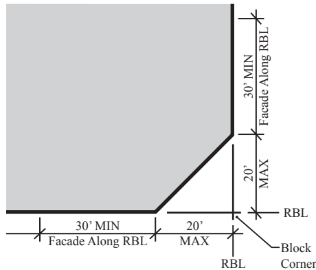
CHAMFERED CORNER
