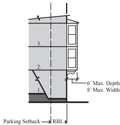
BAY WINDOWS
