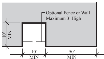
FORECOURT
